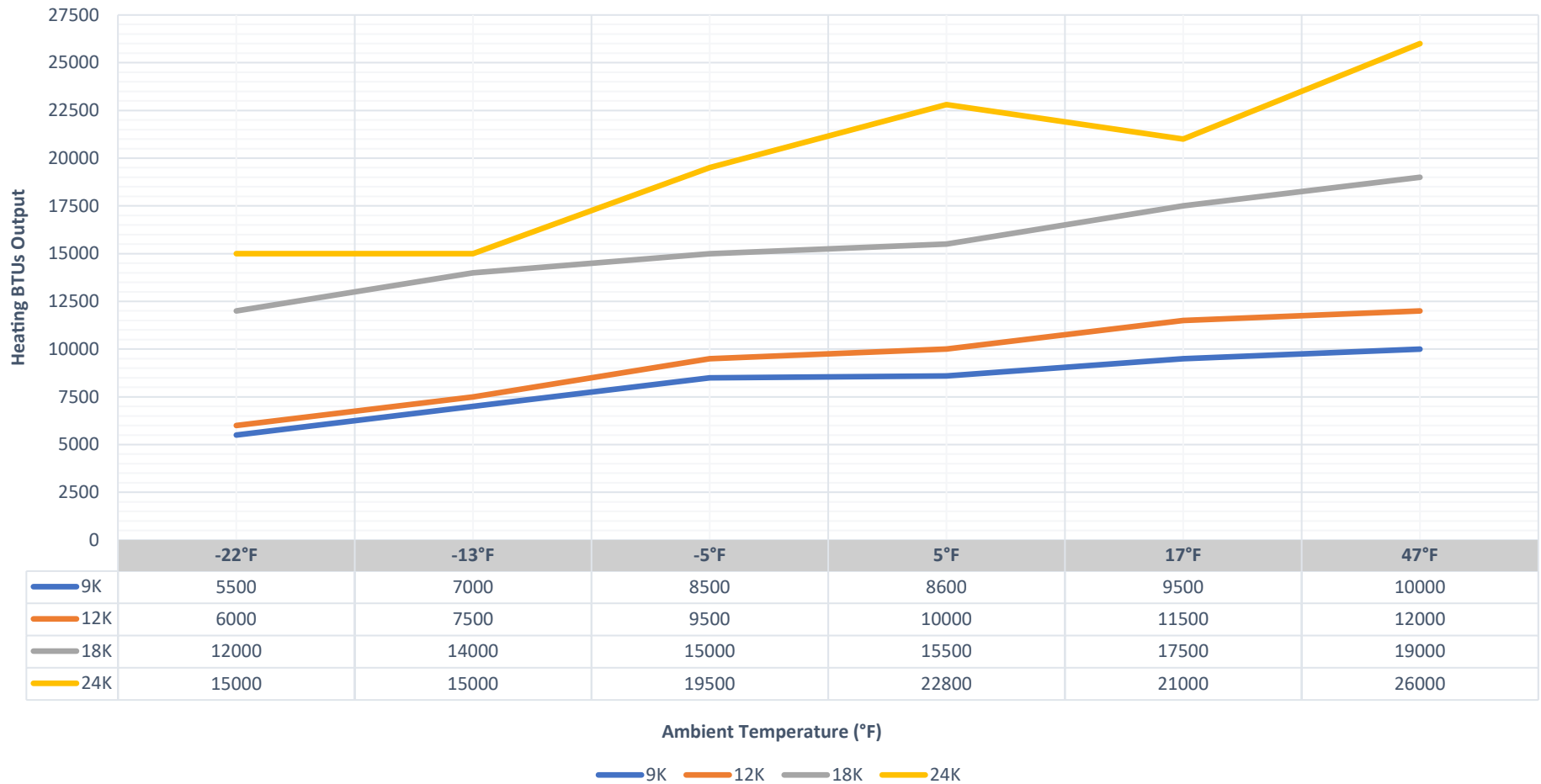
Heating BTU Output at Various Ambient Temperatures
